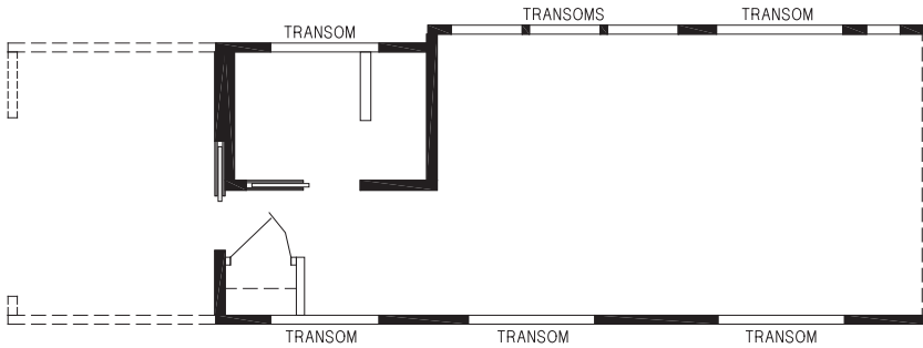
OPTION CLERESTORY
