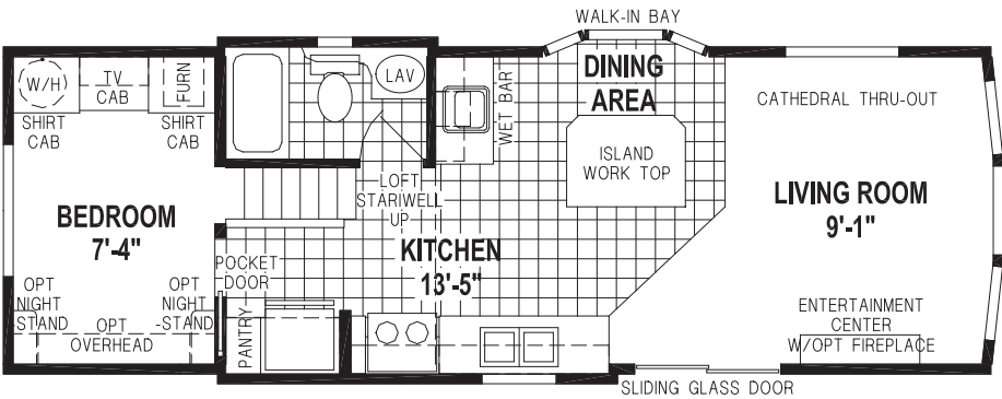
1963CTP/33'-9"12 1BEDROOM - CATHEDRAL THRU-OUT * 1963CTM/33'-9"12
