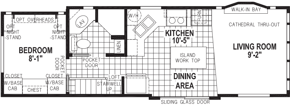
1966CTP/3512 1BEDROOM - CATHEDRAL THRU-OUT
