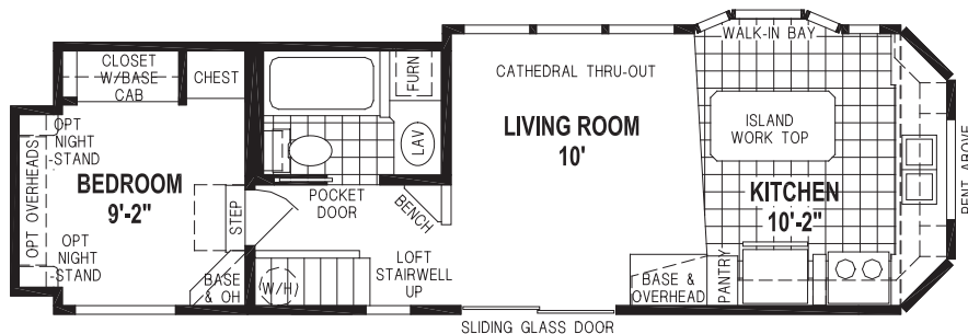
1941CTQ/34'-10"12 1BEDROOM - DROP LOFT - CATHEDRAL THRU-OUT
