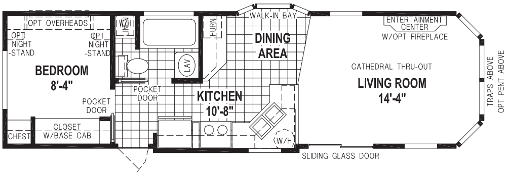
1934CTA/36'-10"12 1BEDROOM - CATHEDRAL THRU-OUT *1934CTA/36'-10"12
