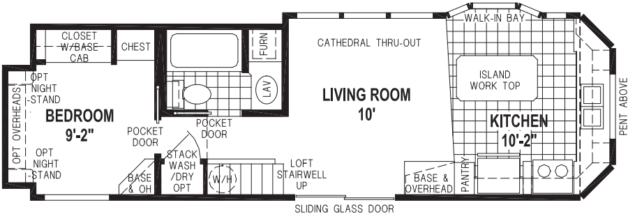
1941CTR/34'-10"12 1BEDROOM - CATHEDRAL THRU-OUT
