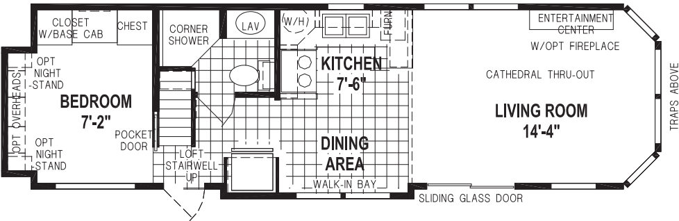
1935CTP/3612 1BEDROOM - CATHEDRAL THRU-OUT
