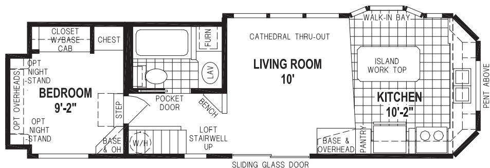
1941CTP/34'-10"12 1BEDROOM - DROP LOFT - CATHEDRAL THRU-OUT
