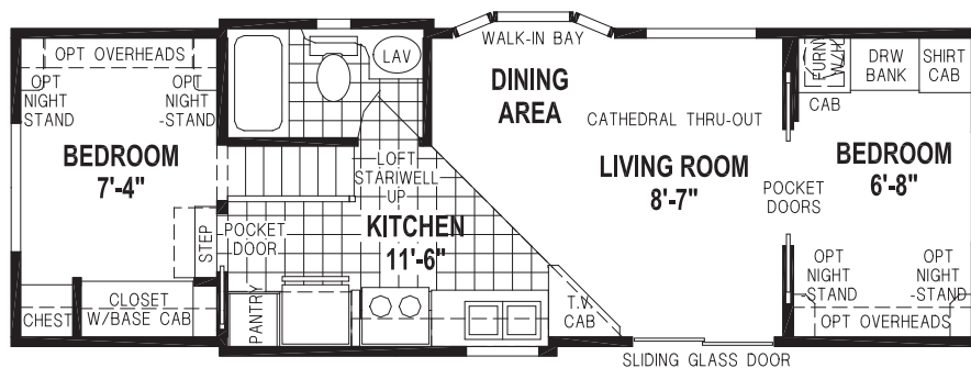
1943CTP/34'-1"12 2BEDROOM - DROP LOFT - CATHEDRAL THRU-OUT (NOT AVAILABLE WITH HOLDING TANKS)
