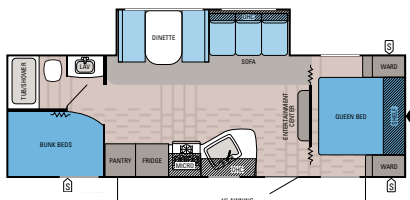
JAY FEATHER | 25BH Ext. Length: TBD Ext. Height: TBD Unloaded Wt. (lbs.): TBD Sleeps: 8-10
