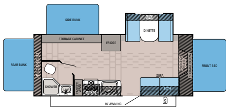
JAY FEATHER | X23F Ext. Length: 24' 10" Ext. Height: 123" Unloaded Wt. (lbs.): 4,400 Sleeps: 8-10
