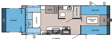
JAY FEATHER | X254 Ext. Length: 27' 4" Ext. Height: 122" Unloaded Wt. (lbs.): 4,705 Sleeps: 8
