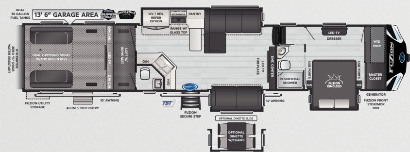
429 WEIGHT 16018 LENGTH 44' 11"
