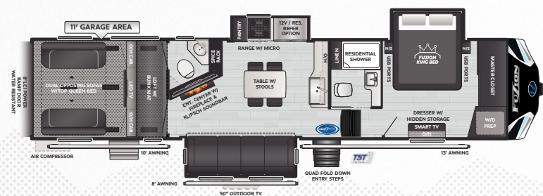
373 WEIGHT 14300 LENGTH 39' 0"
