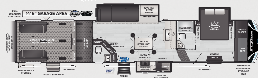
427 WEIGHT 15820 LENGTH 44' 11"
