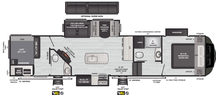
WEIGHT 11485 LENGTH 39' 7"
