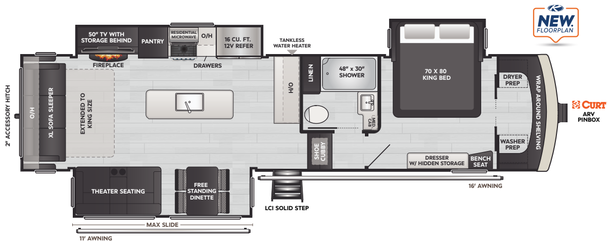
3260RL | WEIGHT 11149 | LENGTH 36' 6"
