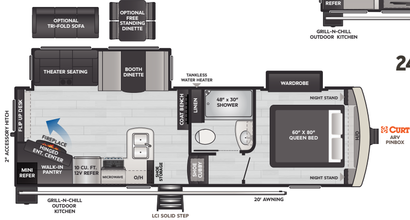
248SLRE | WEIGHT 8143 | LENGTH 28' 11"
