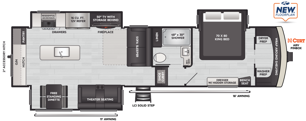
3140RK | WEIGHT 10855 | LENGTH 35' 10"
