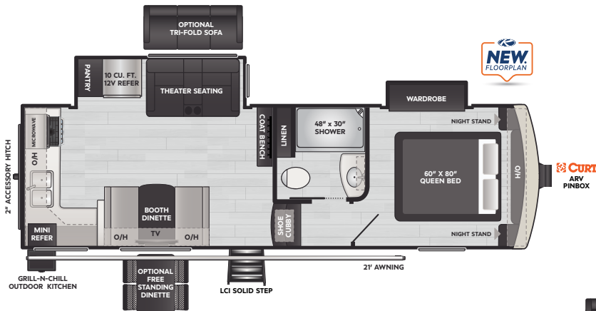
242SLMD | WEIGHT 7690 | LENGTH 28' 6"
