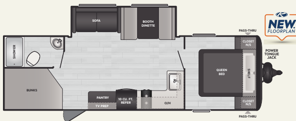
269DBCWE | WEIGHT TBD | LENGTH 30' 8"
