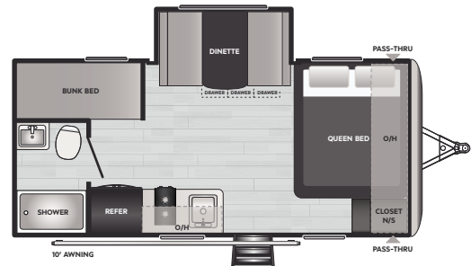
1760BH | WEIGHT 3796 | LENGTH 20' 11"
