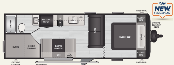
260BHC | WEIGHT 5069 | LENGTH 20' 11"
