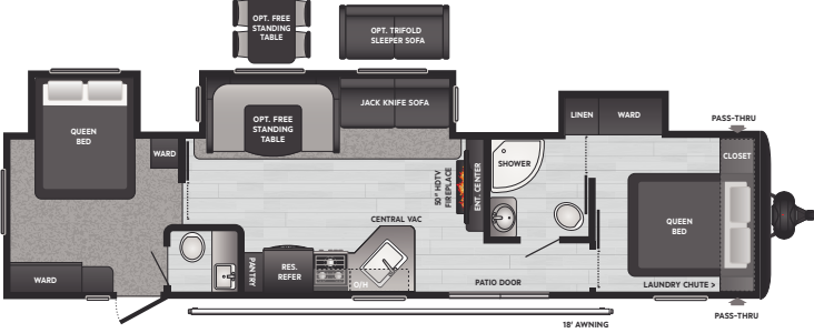
38FQ | WEIGHT 9350 | LENGTH 39' 11"
