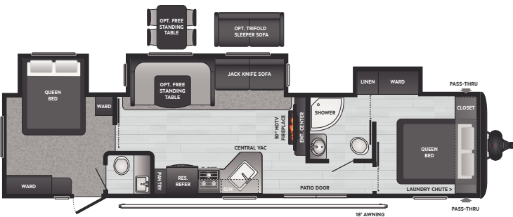
38FQ | WEIGHT 9246 | LENGTH 39' 11"
