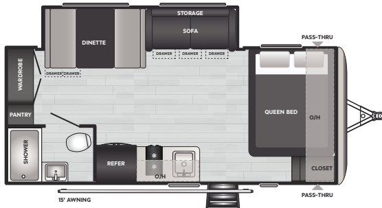
1860SS | WEIGHT 4100 | LENGTH 22' 10"
