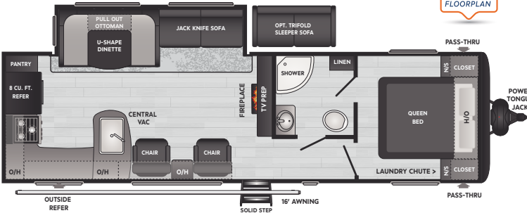
280RKWE | WEIGHT TBD | LENGTH TBD
