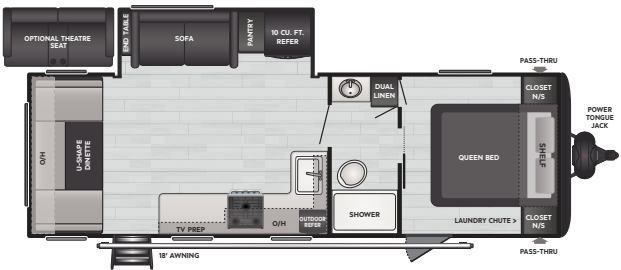
256RD | WEIGHT 6225 | LENGTH 29' 5"
