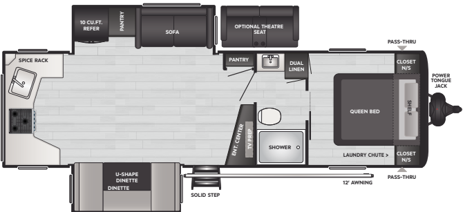
281RK | WEIGHT 7395 | LENGTH 32' 5"
