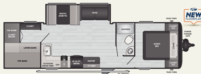
291BRC | WEIGHT 6795 | LENGTH 33' 11"
