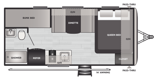
1800BH | WEIGHT 3036 | LENGTH 20' 6"
