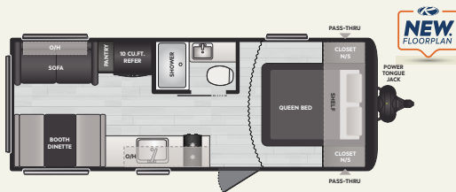
200RLCWE | WEIGHT 4534 | LENGTH 25' 1"
