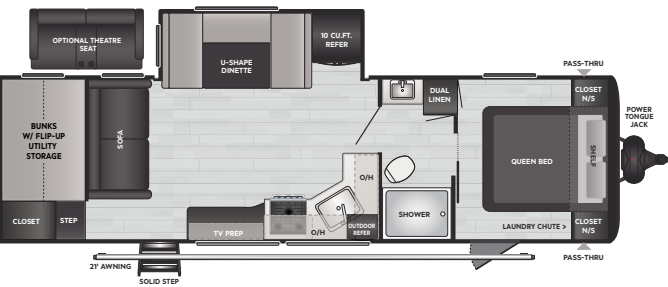
286BHU | WEIGHT 6895 | LENGTH 33' 1"
