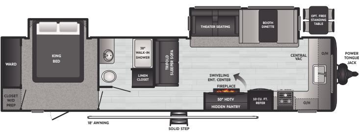
34FK | WEIGHT 8490 | LENGTH 38' 11"
