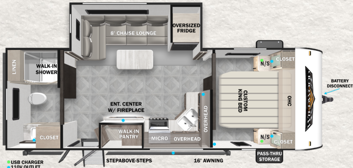
MODEL #: 22RBS HITCH: 765 LBS UVW: 5,928 LBS LENGTH: 26'11"
