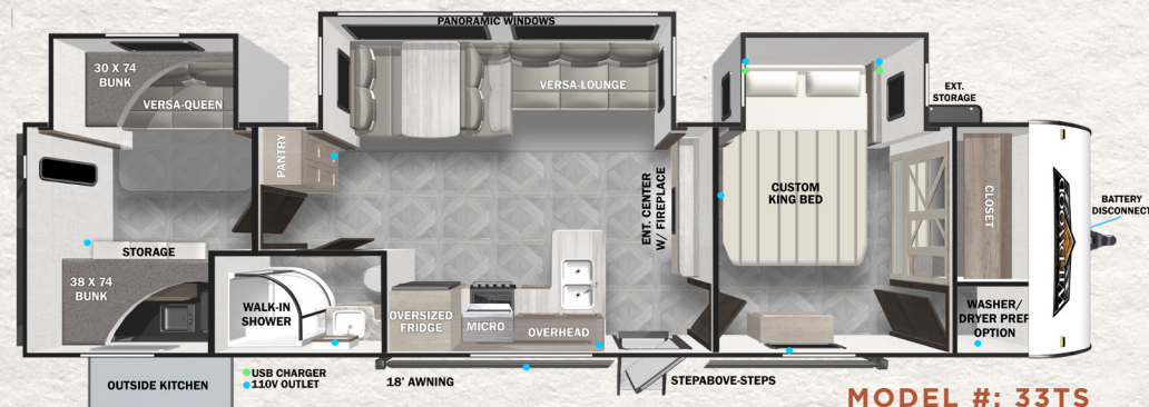
MODEL #: 33TS HITCH: 1,088 LBS UVW: 9,276 LBS LENGTH: 38'9"
