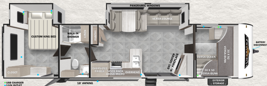
MODEL #: 36VBDs HITCH: 1,155 LBS UVW: 8,533 LBS LENGTH: 38'11"
