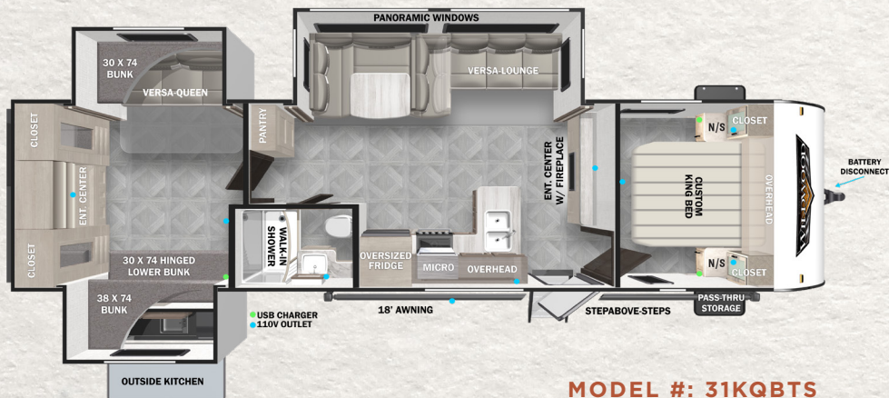
MODEL #: 31KQBTs HITCH: 905 LBS UVW: 8,573 LBS LENGTH: 36'7"
