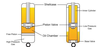
BILSTEIN'S MONOTUBE | vs. | COMPETITOR'S DUALTUBE
