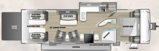
291SLC/293GSLR (16' CARGO)
