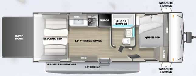
211SLC (13' 4" CARGO)
