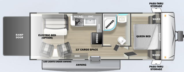
241 SPORT (13' CARGO)
