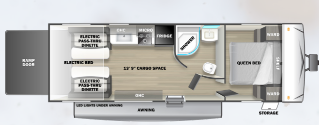
242SLC AVAILABLE AS 242GSLC (FIBERGLASS) (13' 9" CARGO)
