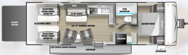
251SLC AVAILABLE AS 251GSLC (FIBERGLASS) (14' 4" CARGO)
