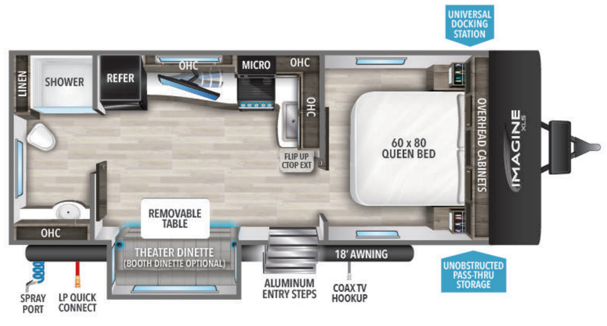
22RBE UVW † 5,125 HITCH † 497 LENGTH † 25' 11" HEIGHT 10' 10" CAPACITY 43 82 37
