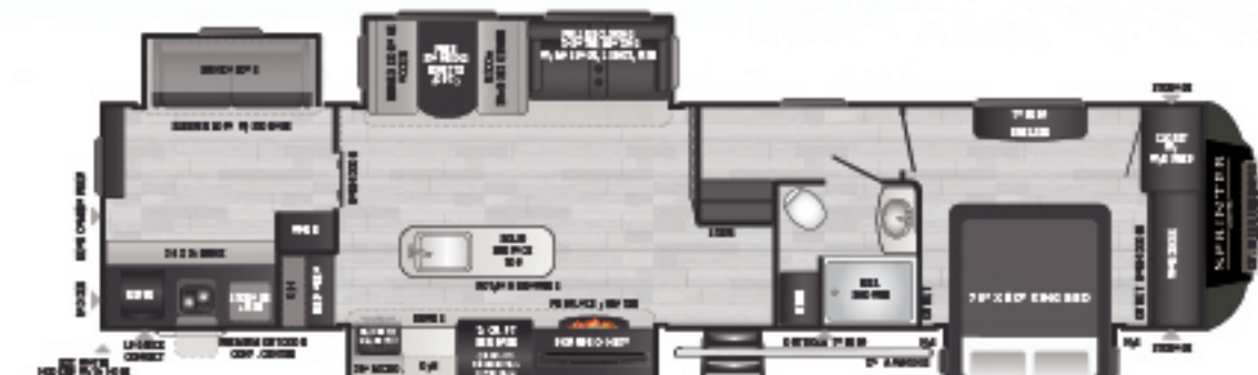
3620LBH | Luxury bunk, open concept living area WEIGHT 11817 LENGTH 40' 6"
