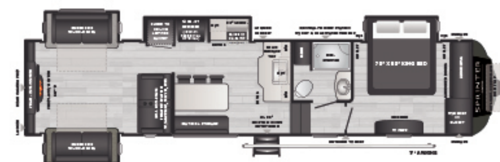
3530DEN | Rear den w/ bartop, dual tri-fold sleeper sofas, theater seating WEIGHT 10912 LENGTH 39' 0"
