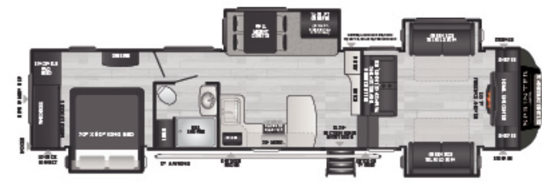
NEW! 3670FLS | Front living, stackable W/D prep WEIGHT 11755 LENGTH 40' 6"
