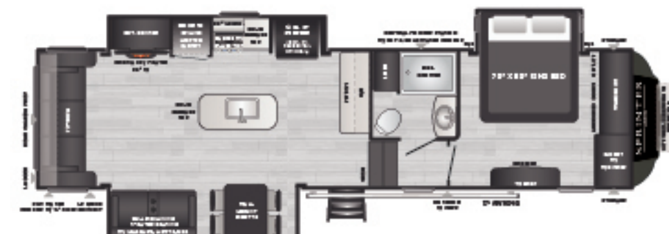
3190RLS | Rear living, full pantry, huge entertainment WEIGHT 10461 LENGTH 35' 11"
