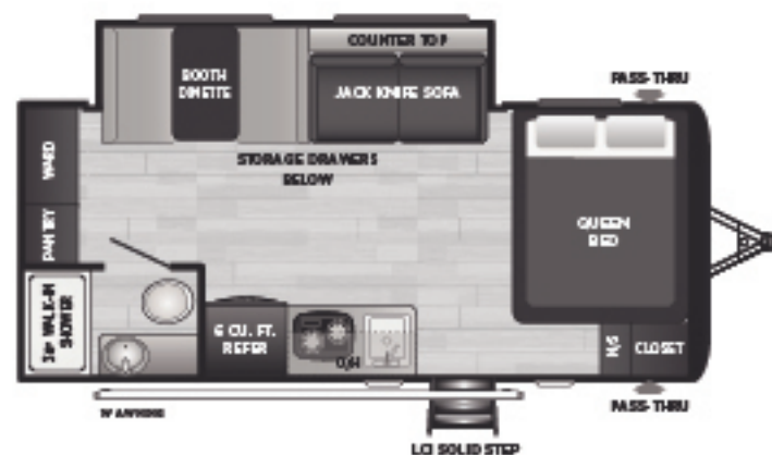
186SS | Single-axle, one slide, large pantry/ward WEIGHT 4160 LENGTH 22' 10"
