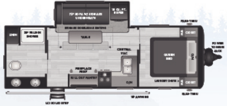
243RB | Rear bath, dual vanities, 72" jack-knife system WEIGHT 5957 LENGTH 28' 8"
