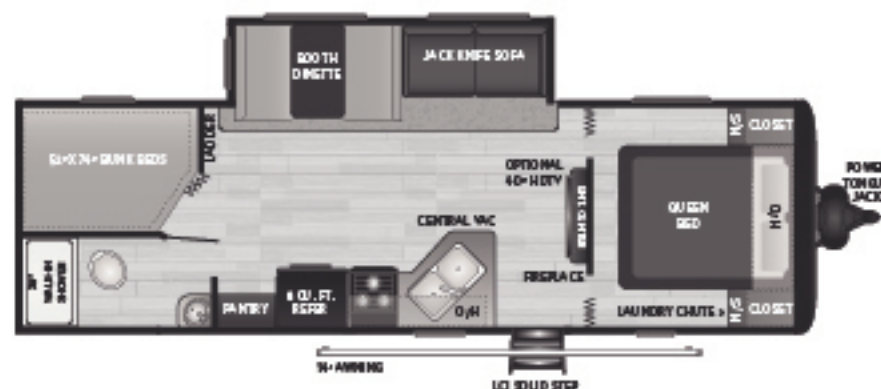
26BHWE One slide, double-over-double bunkhouse WEIGHT 5927 LENGTH 30' 4"
