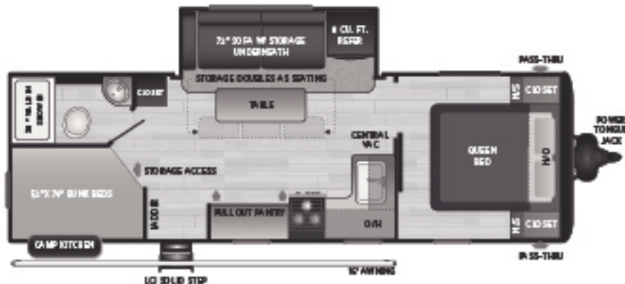
NEW! 25DBWE One slide, double-over-double bunks, camp kitchen WEIGHT 6180 LENGTH 29' 11"
