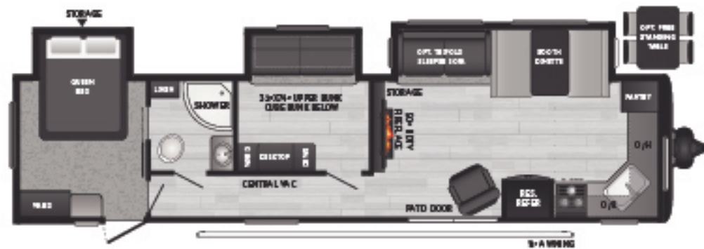
38FKTS | Triple slide w/ bed slide, mid-bunkhouse, patio door WEIGHT 9079 LENGTH 39' 11"
