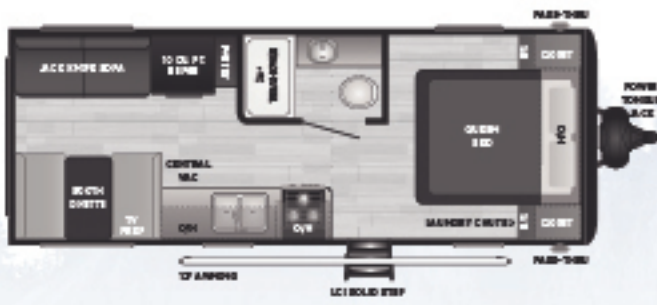
202RD | Non-slide, rear dinette, large rear window WEIGHT 4508 LENGTH 24' 11"
