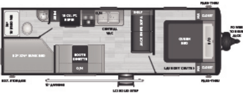
262BH | Non-slide, double-over-double bunkhouse WEIGHT 4989 LENGTH 29' 3"
