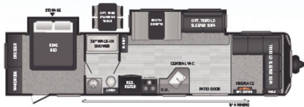
38FDDS | Double slide w/ bed slide, front sectional, patio door WEIGHT 8277 LENGTH 39' 11"
