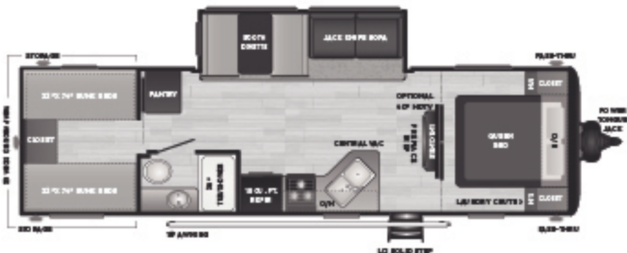
290QB | One slide, quad bunk, wrap-around rear storage WEIGHT 6604 LENGTH 33' 3"
