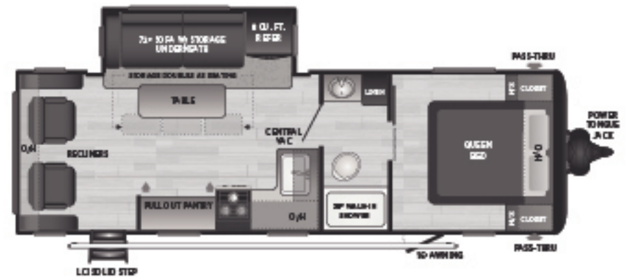
25RLWE One slide, rear living w/ recliners, hidden pantry, 50" HDTV WEIGHT 5970 LENGTH 29' 11"
