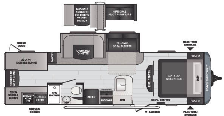
292BHWE | Couple's coach w/ oversized dinette
