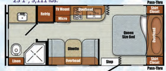
23BHS 26'1"; 4,203 lbs.
