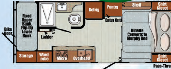
19CSK 23'1"; 3,009 lbs.
