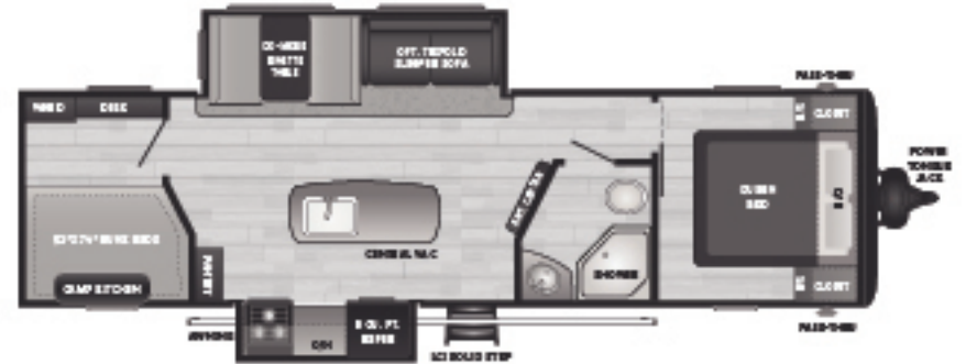
30BHKSWE | Two slides, private bunkhouse, kitchen island, camp kitchen Weight: 7462 lbs. | Length: 34' 11"
