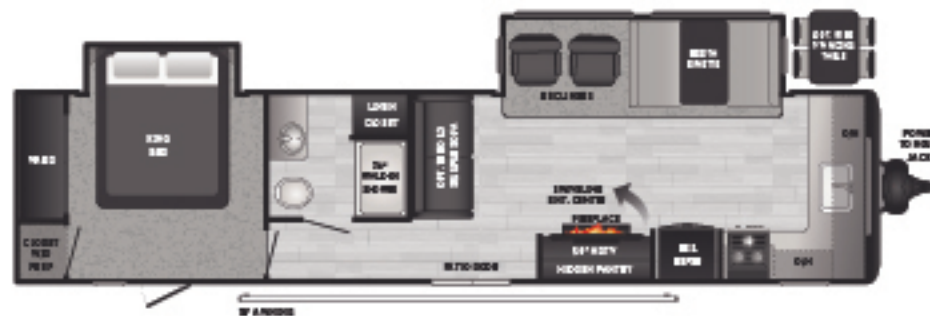
34FKDS | Front kitchen, hidden pantry, w/d prep, patio door Weight: 8293 lb | Length: 38' 11"
