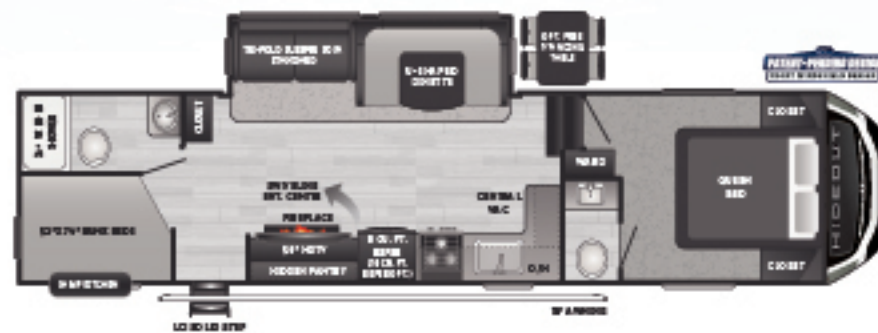
301DBS | One slide, double-over-double bunks, hidden pantry, 1 1/2 baths Weight: 8669 lb | Length: 34' 2"
