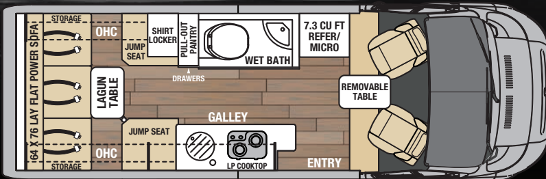
20C - Power Sofa with Double Captains Chairs
