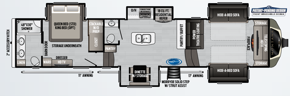
3760/3761FL | FRONT LIVING W/ FULL BATH AND A HALF | Weight: 14147 LBS. | Length: 41' 0" RV REFRIGERATOR RES. REFRIGERATOR
