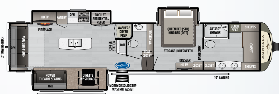
3930/3931FB | FRONT BATHROOM W/ FRONT WARDROBE | Weight: 13564 LBS. | Length: 41' 4" RV REFRIGERATOR RES. REFRIGERATOR
