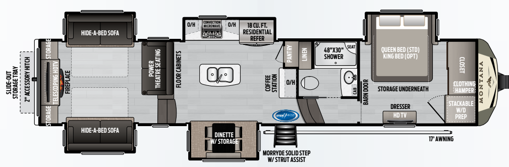
3790/3791RD | ELEVATED REAR DEN W/ REAR PULL-OUT STORAGE | Weight: 14119 LBS. | Length: 40' 4" RV REFRIGERATOR RES. REFRIGERATOR
