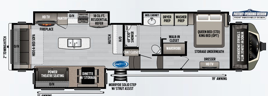
3810/3811MS | REAR LIVING ROOM W/ MASTER SUITE WALK-THROUGH CLOSET | Weight: 13595 LBS. | Length: 40' 9" RV REFRIGERATOR RES. REFRIGERATOR
