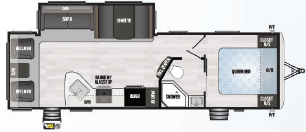
271RLWE | LARGE SLIDE, REAR LIVING, CHAIRS, DUAL ENTRANCE Weight: 6687 LBS. | Length: 31' 10"
