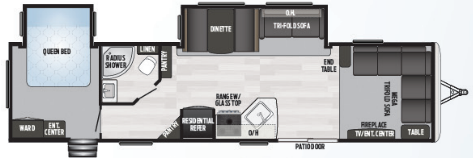
38FL | AMAZING FRONT LOUNGE, FIREPLACE, ENTERTAINMENT-FOCUSED Weight: 8641 LBS. | Length: 38' 11"
