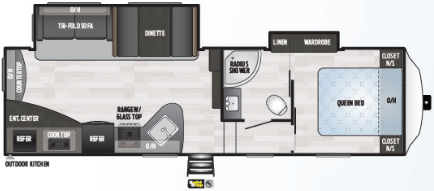
272FWRE | 2 SLIDES, REAR ENTERTAINMENT, OUTSIDE KITCHEN Weight: 7846 LBS. | Length: 30' 2"
