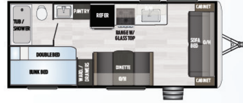
189FLWE | NON SLIDE, FRONT LIVING Weight: 4228 LBS. | Length: 23' 7"
