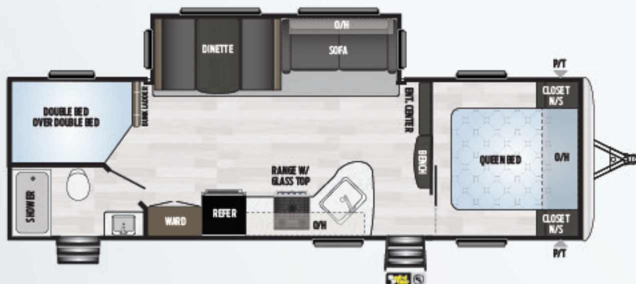
282BHWE | LARGE SLIDE, DOUBLE BUNKS, PRIVATE BEDROOM Weight: 6730 LBS. | Length: 32' 1"
