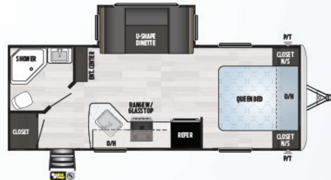
212RBWE | SMALL SLIDE, REAR BATH Weight: 5239 LBS. | Length: 25' 11"
