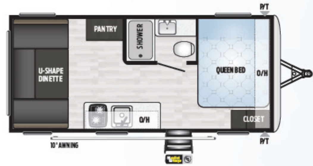
1750RD | REAR DINETTE, INCREDIBLE COUNTERTOP SPACE Weight: 3414 LBS. | Length: 21' 5"
