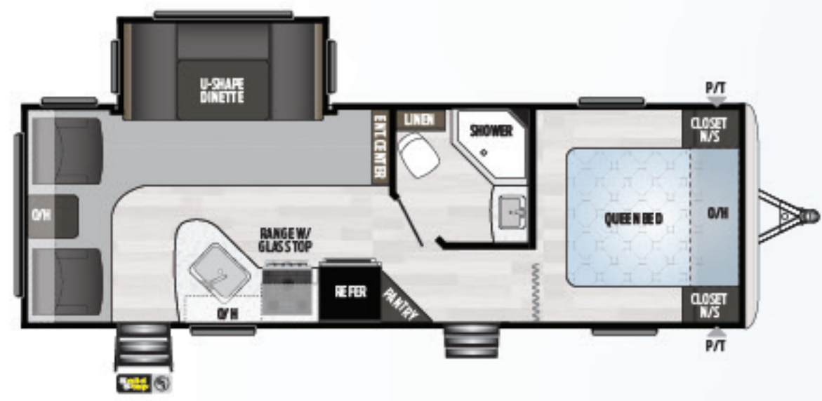
258RLWE | SMALL SLIDE, REAR LIVING, CHAIRS Weight: 5959 LBS. | Length: 29' 7"
