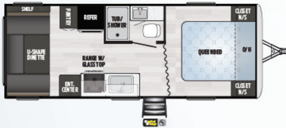
202QBWE | NON SLIDE, QUEEN BED Weight: 4278 LBS. | Length: 24' 10"
