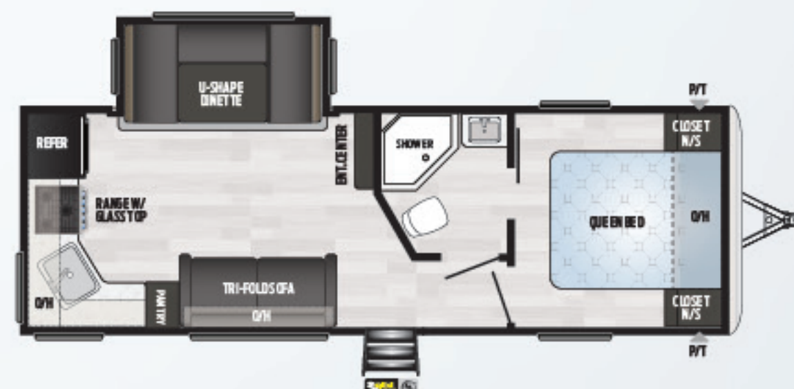
242RKWE | SMALL SLIDE, REAR KITCHEN, DUAL ENTRY BATH Weight: 5729 LBS. | Length: 28' 6"
