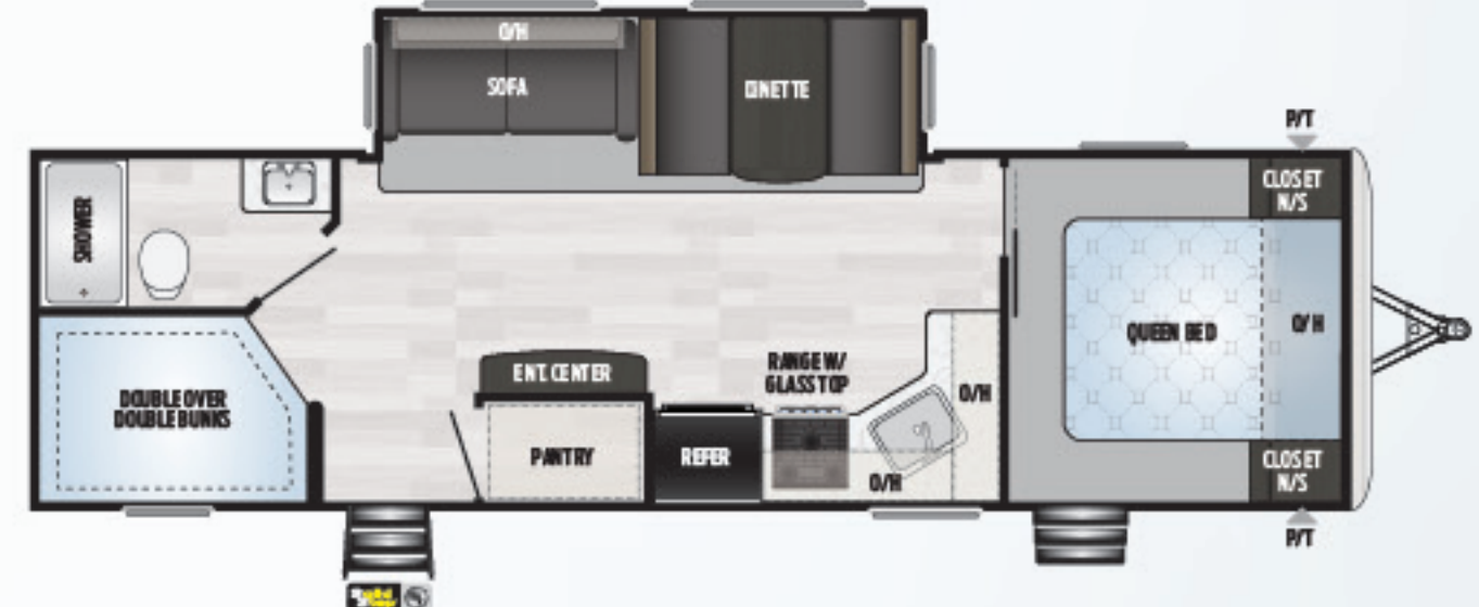
280BHWE | LARGE SLIDE, WALK-IN PANTRY, DOUBLE BUNKS, DUAL ENTRANCE Weight: 6945 LBS. | Length: 32' 11"
