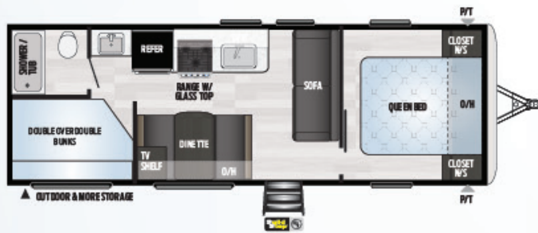
260TBWE | NON SLIDE, DOUBLE BUNKS, PRIVATE BEDROOM Weight: 4872 LBS. | Length: 28' 6"
