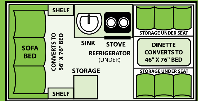
RANGER 12 FLOOR PLAN
