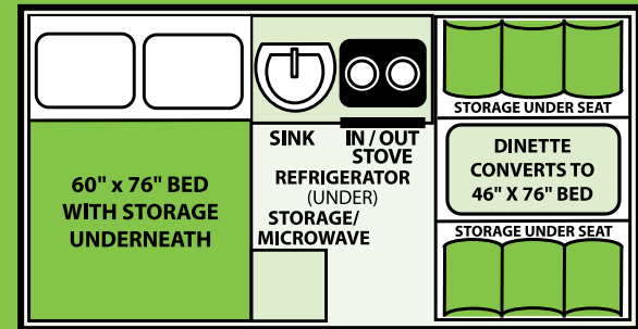
CLASSIC FLOOR PLAN - PERMANENT BED
