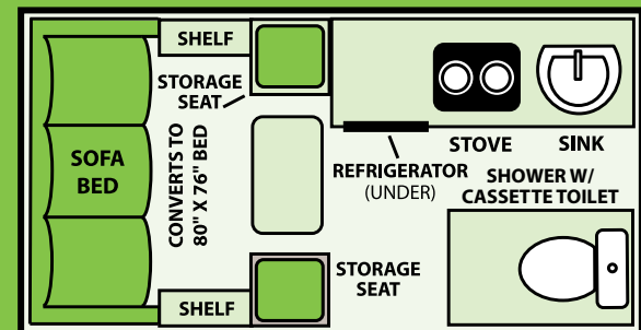
LXE FLOOR PLAN
