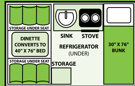
TITANIUM 10 FLOOR PLAN
