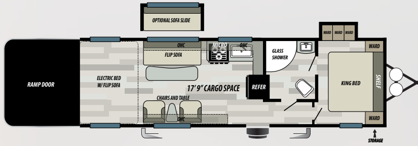
FK2917G DRY WEIGHT 9,108 LBS
