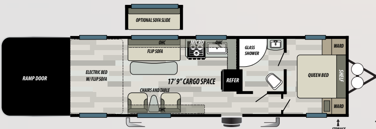
FQ2817 DRY WEIGHT 8,212 LBS
