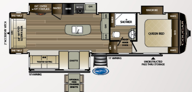
30RLS | Rear living room, gourmet kitchen Weight: 8890 LBS. | Length: 33'6"
