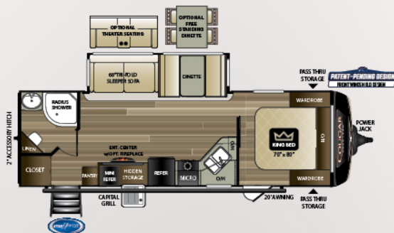
26RBS | Rear bath, slide and outside kitchen Weight: 6525 LBS. | Length: 29' 11"
