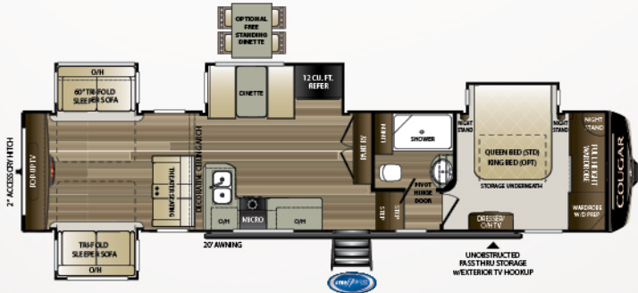
366RDS | Rear den, four slides Weight: 11202 LBS. | Length: 39' 4"
