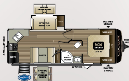
24SABWE | Dual Entry Rear Kitchen with Slide Weight: 5990 LBS. | Length: 28' 4"
