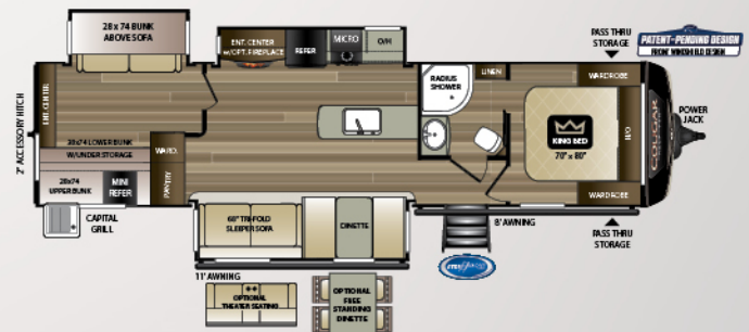
34TSB | Three-slide bunk house w/ outside kitchen Weight: 8548 LBS. | Length: 37' 5"
