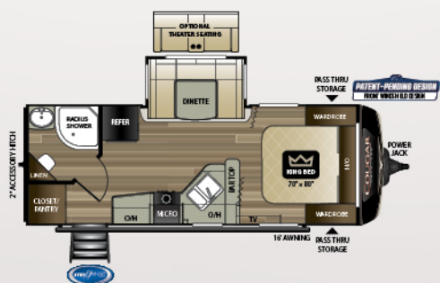
22RBS | Short, rear bath w/ slide Weight: 5590 LBS. | Length: 25' 11"
