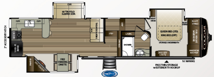
338RLK | Rear living room, outside kitchen Weight: 10605 lbs. | Length: 36' 5"
