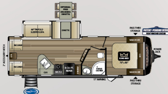
27SAB | Rear living room, side-aisle bath Weight: 6651 LBS. | Length: 31' 5"
