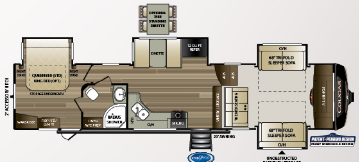
367FLS | Front living room w/ windshield Weight: 10963 LBS. | Length: 39' 4"
