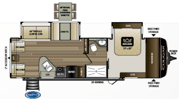
29RLD | Rear living room, bed slide w/ large front closet Weight: 7320 LBS. | Length: 34'
