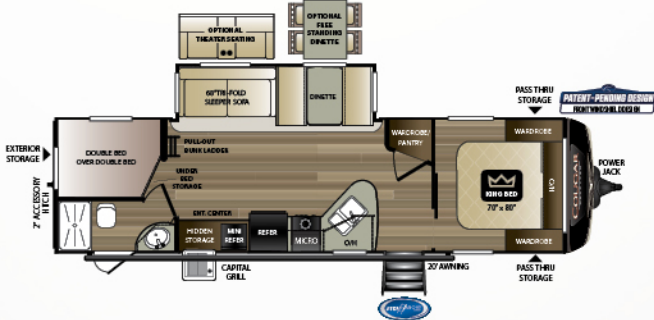
29BHS | Double bunkhouse, outside kitchen Weight: 6975 LBS. | Length: 34' 1"
