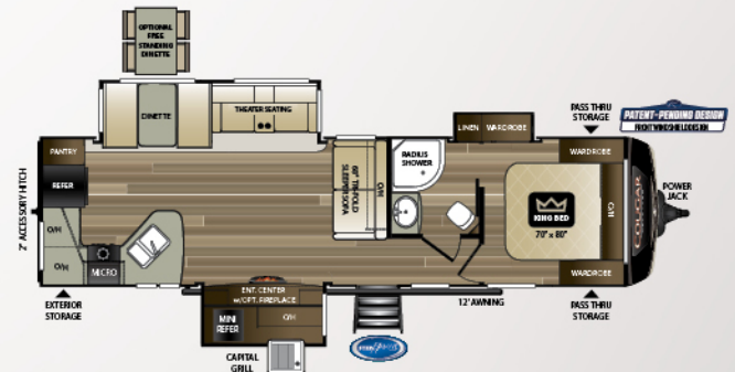
33MLS | Rear kitchen, outside kitchen Weight: 8088 LBS. | Length: 35' 3"
