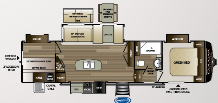
32DBH | Double bunkhouse w/ extra storage Weight: 9300 LBS. | Length: 35'5"
