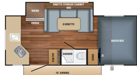
HUMMINGBIRD | 17RK Ext. Length: 19' 9" Travel Ht: 110" Unloaded Wt. (lbs): 2,985 Sleeps: 3-4
