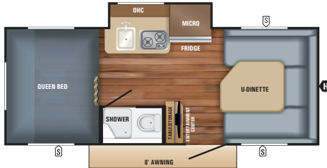
HUMMINGBIRD | 16FD Ext. Length: 18' 10" Travel Ht: 111" Unloaded Wt. (lbs): 2,535 Sleeps: 3-4
