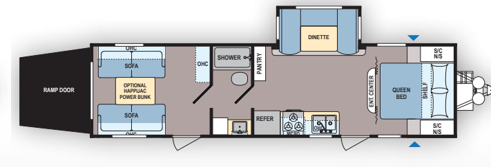
Lantern SUT | 300TQ Ext. Length: 34' 10" Ext. Height: 12' 4" Average Shipping Weight: 6,838 Sleeps 8 Eastern Region production**
