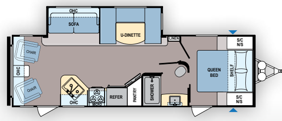
Lantern | 270RLWE Ext. Length: 30' 8" Ext. Height: 11' 2" Average Shipping Weight: 6,008 Sleeps 4-5
