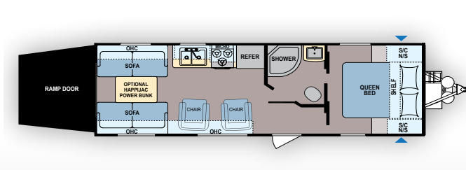
Lantern SUT | 250TQ Ext. Length: 29' 7" Ext. Height: 11' 4" Average Shipping Weight: 5,514 Sleeps 6 Eastern Region production**
