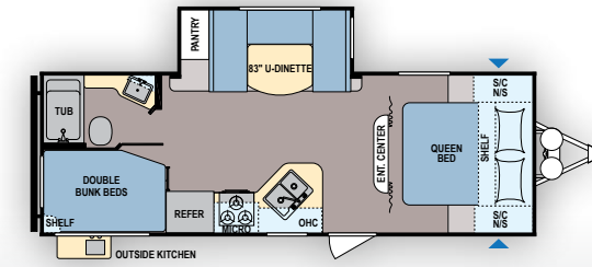
Lantern | 244BHWE Ext. Length: 27' 7" Ext. Height: 11' 4" Average Shipping Weight: 5,500 Sleeps 6-8
