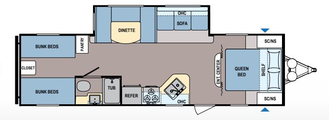
Lantern | 295QBWE Ext. Length: 32' 8" Ext. Height: 11' 3" Average Shipping Weight: 6,283 Sleeps 8-9
