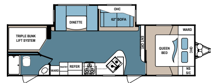
DENALI TRAVEL TRAILER | 2611BH Ext. Length: 33' 10" Ext. Height: 10' 11" Average Shipping Weight: 7,198 Sleeps: 5-7
