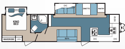
DENALI TRAVEL TRAILER | 350FK Ext. Length: 38' 7" Ext. Height: 11' 7" Average Shipping Weight: 8,413 Sleeps: 6
