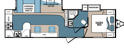
DENALI TRAVEL TRAILER | 289RK Ext. Length: 34' 8" Ext. Height: 11' 2" Average Shipping Weight: 7,746 Sleeps: 3-4
