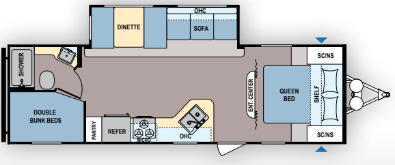
Lantern | 262BHWE Ext. Length: 30' 7" Ext. Height: 11' 4" Average Shipping Weight: 5,880 Sleeps 8-10
