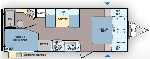
Lantern | 215BHWE Ext. Length: 25' 11" Ext. Height: TBD Average Shipping Weight: TBD Sleeps 5-7
