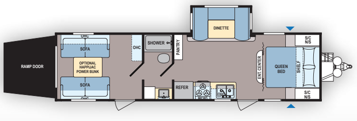
Lantern SUT | 300TQ Ext. Length: 34' 10" Ext. Height: 12' 4" Average Shipping Weight: 6,838 Sleeps 8 Eastern Region production**
