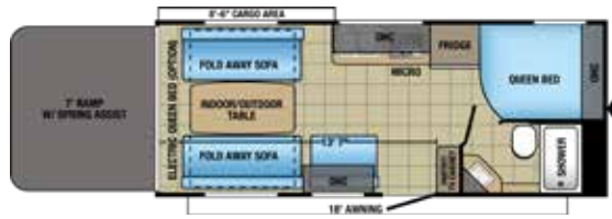
OCTANE SUPER LITE | 222 Ext. Lgth: 26' 5" Ext. Ht: 134" Unloaded Wt (lbs.): 5,350 Sleeps: 6
