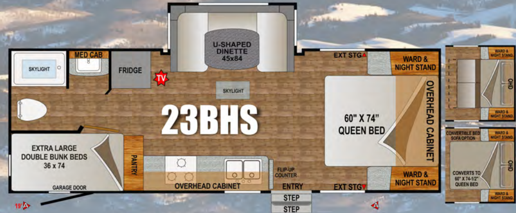
DRY WEIGHT: TBA ~ FLOOR LENGTH: 24'
