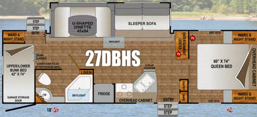
DRY WEIGHT: TBA ~ FLOOR LENGTH: 28'
