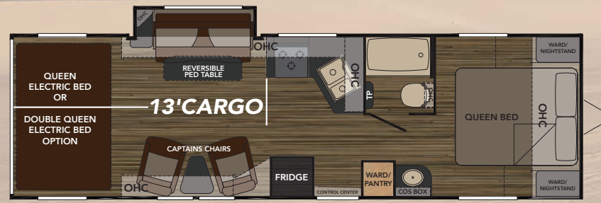
FS2700/13 SHOWN WITH OPTIONAL SLIDE OUT & BAY WINDOW
