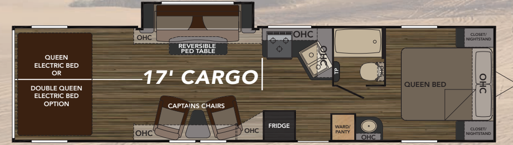
FS3100/17 SHOWN WITH OPTIONAL SLIDE OUT & BAY WINDOW
