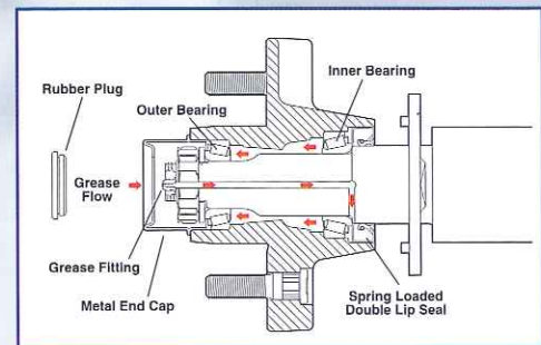
Easy lube axles can be lubricated without removing the wheel.
