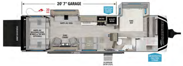
30G 20' 7" GARAGE UVW' EMPTY HITCH' GVWR LENGTH' HEIGHT CAPACITY 9,139 1,425 13,000 34' 10" 12' 4" 90 76 37
