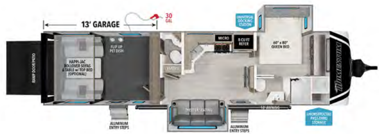
31G 13' GARAGE UVW' EMPTY HITCH' GVWR LENGTH' HEIGHT CAPACITY 8,975 1,600 13,000 35' 11" 12' 4" 90 37 39 37* * 1/2 BATH DOUBLES AS BLACK/GREY
