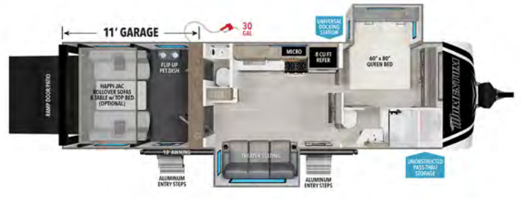
29G 11' GARAGE UVW' EMPTY HITCH' GVWR LENGTH' HEIGHT CAPACITY 9,278 1,592 13,000 33' 11" 12' 4" 90 37 39 37* * 1/2 BATH DOUBLES AS BLACK/GREY
