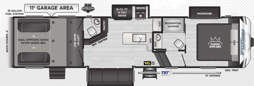
337 | WEIGHT 12795 | LENGTH 36' 7"
