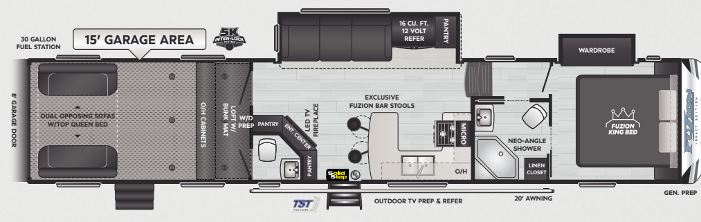
415 | WEIGHT 14154 | LENGTH 44' 0"
