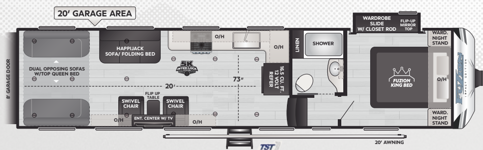
3120 | WEIGHT 11823 | LENGTH 35' 3"
