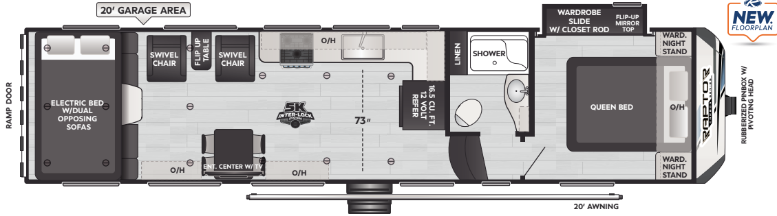
310 | WEIGHT 11270 | LENGTH 35' 3" | WFO
