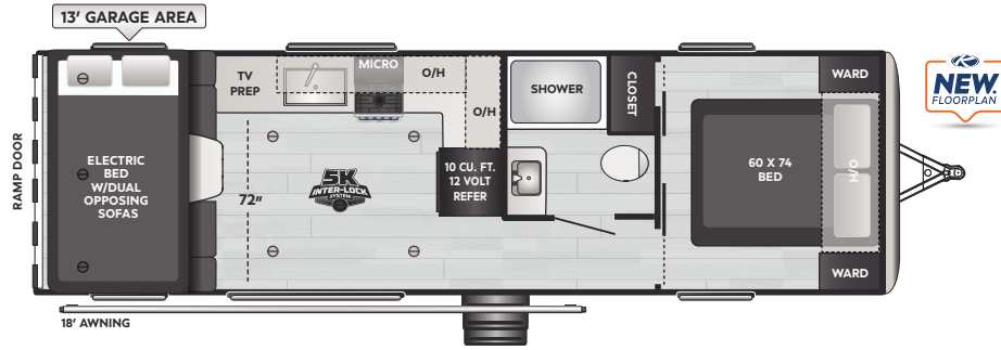
29WFO | WEIGHT TBD | LENGTH 32' 3" | WFO
