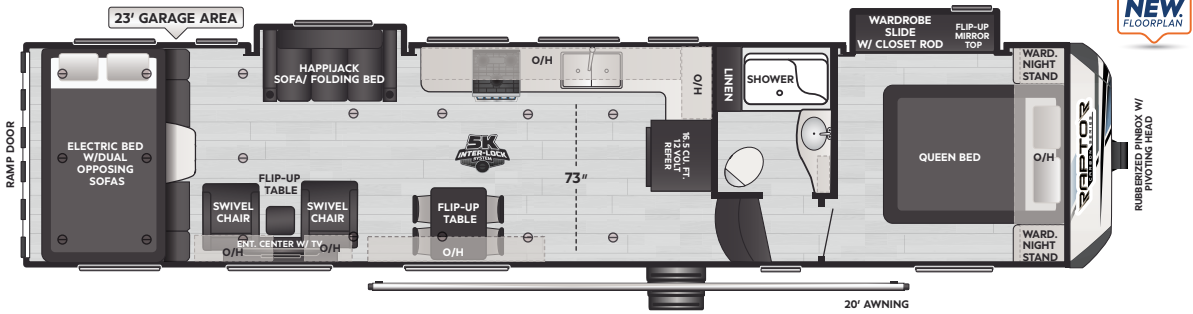
340 | WEIGHT 12035 | LENGTH 38' 3" | WFO
