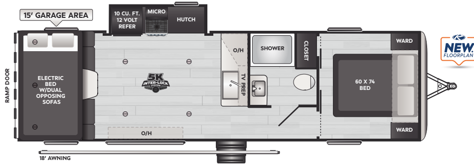
30WFO | WEIGHT 7575 | LENGTH 33' 5" | WFO
