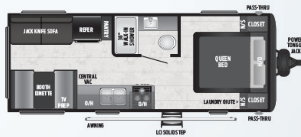
202LHS | NON-SLIDE, REAR DINETTE Weight: 4483 LBS. | Length: 24' 11"
