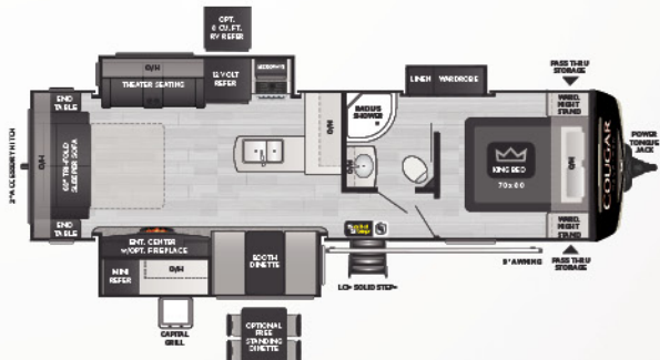
29RLKWE | WEIGHT 7719 | LENGTH 33' 3"
