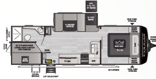
25DBSWE | WEIGHT 6223 | LENGTH 29' 10"
