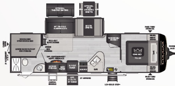
29BHSWE | WEIGHT 7087 | LENGTH 34' 1"
