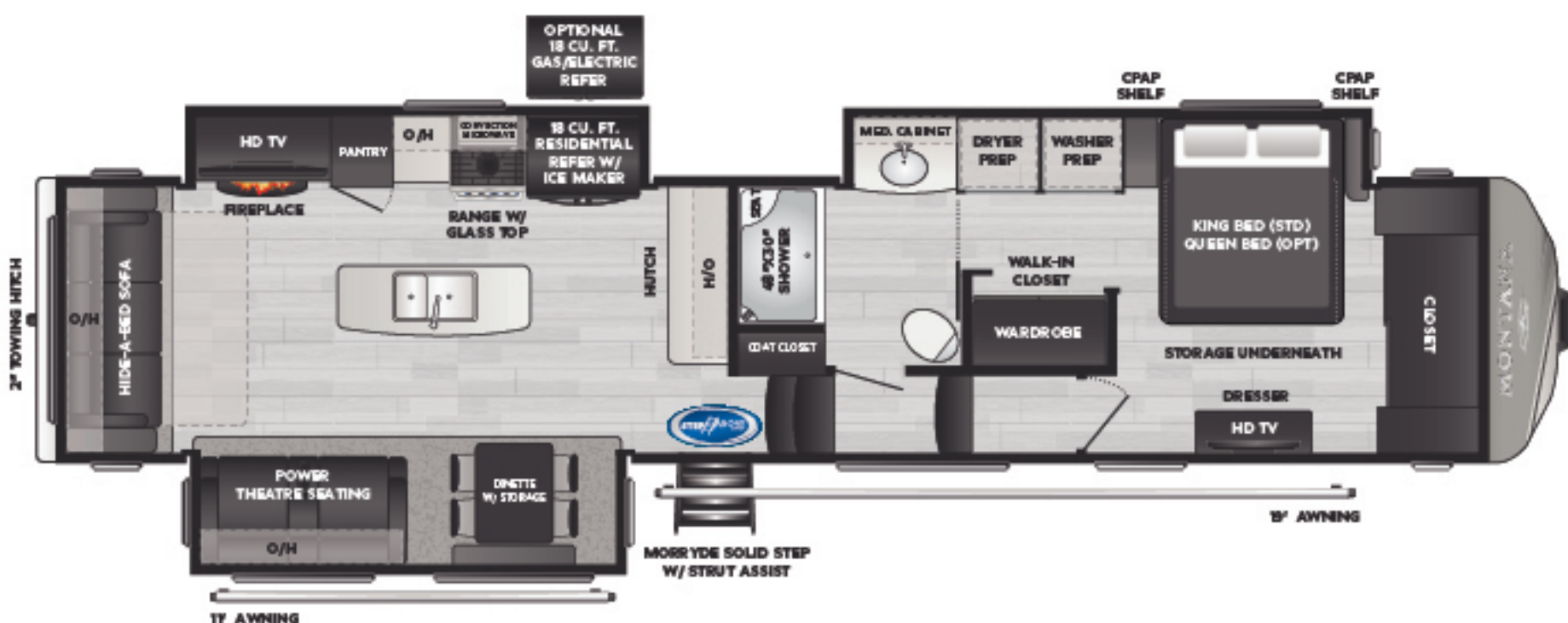
3813MS Rear living room w/ master suite & walk-in closet RESIDENTIAL REFRIGERATOR WEIGHT 13763 LENGTH 40' 9"
