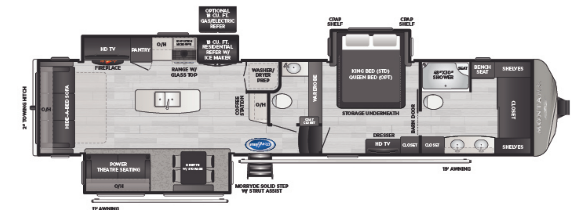
3931FB Front bathroom w/ front wardrobe RESIDENTIAL REFRIGERATOR WEIGHT 13533 LENGTH 41' 4"
