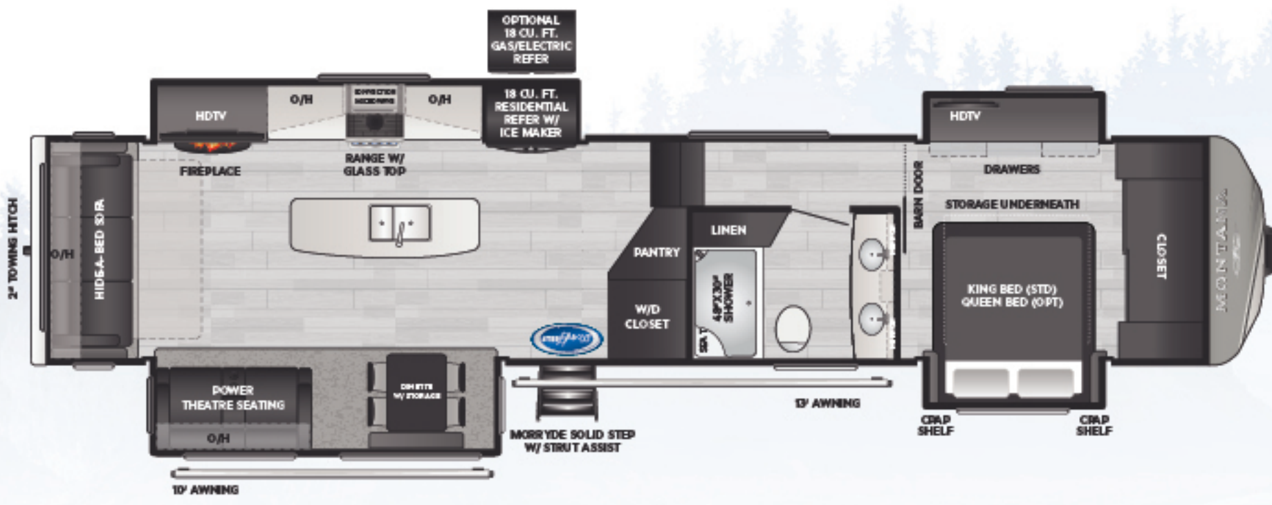
3781RL Rear living w/ double vanity bathroom & double slide bedroom RESIDENTIAL REFRIGERATOR WEIGHT 13485 LENGTH 41' 0"
