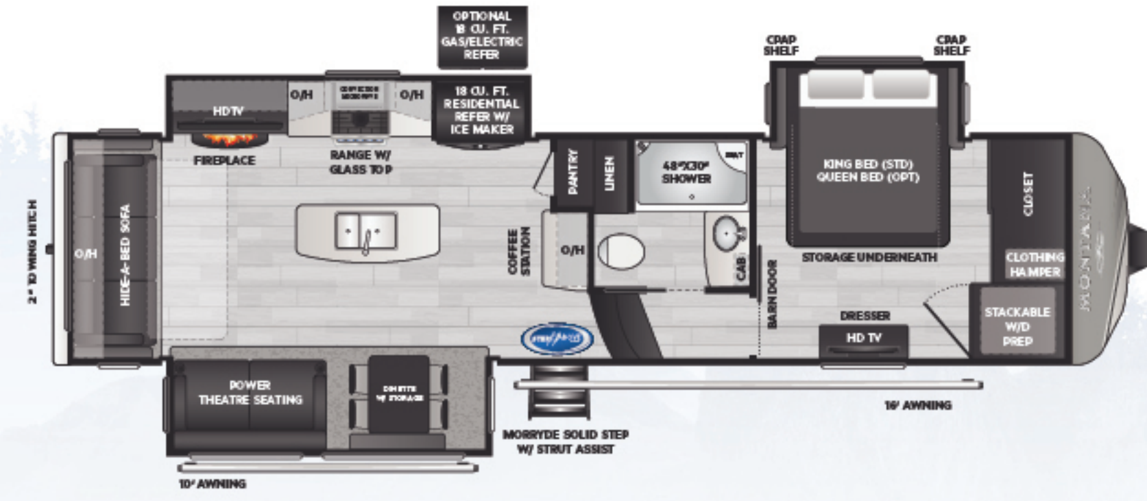
3121RL Rear living room, three slides RESIDENTIAL REFRIGERATOR WEIGHT 12273 LENGTH 35' 0"
