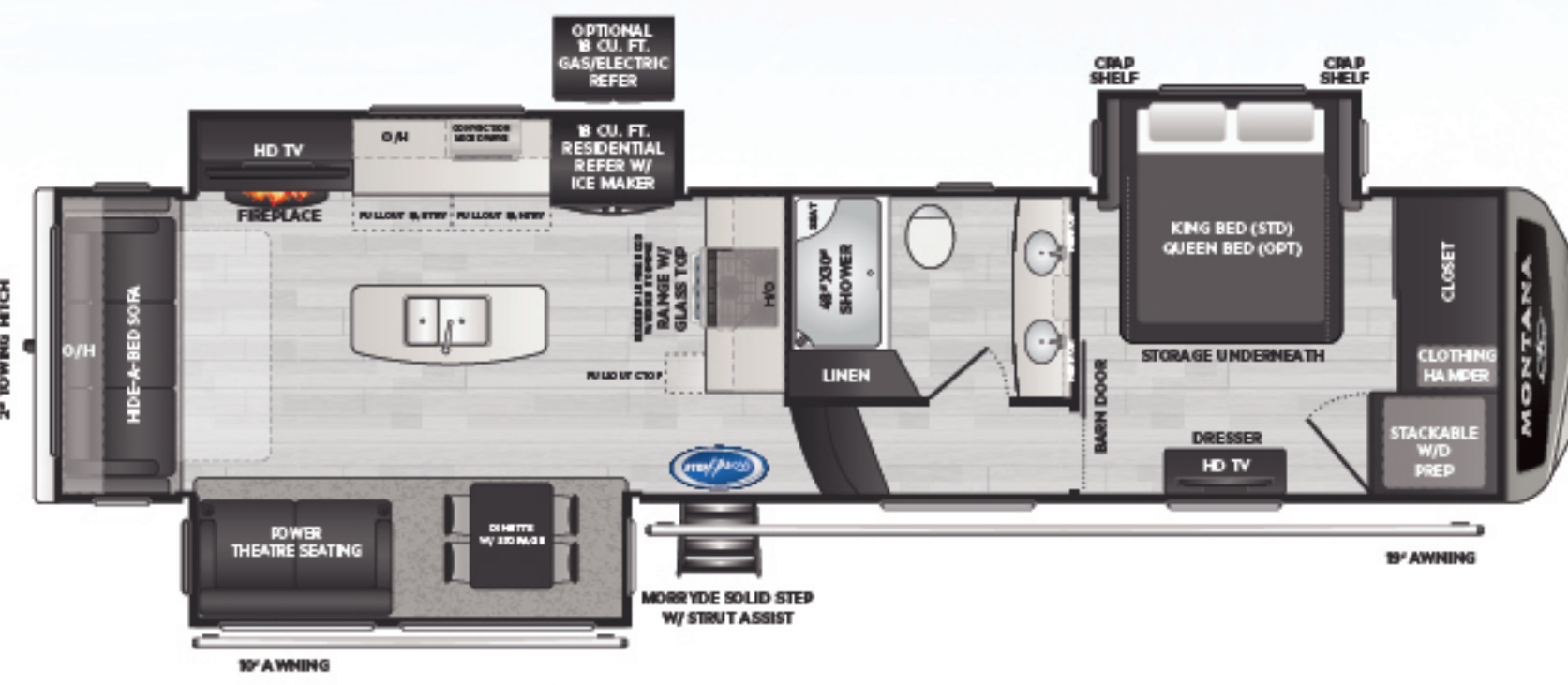
3231CK Center kitchen, three slides, dual vanity RESIDENTIAL REFRIGERATOR WEIGHT 12752 LENGTH 37' 5"
