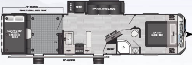
NEW! 35 | Tandem axle, 12' garage, u-shaped kitchen
