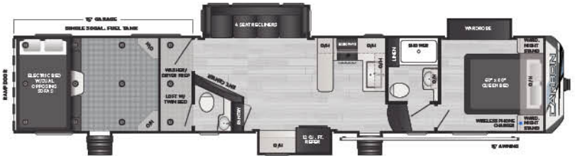
NEW! 418 | Triple axle, 15' garage, u-shaped kitchen
