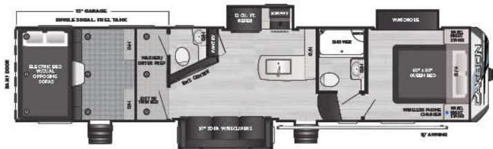
358 | Tandem axle, 13' garage, 1 1/2 bath
