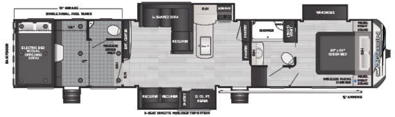
403 | Triple axle, 13' garage, 1 1/2 bath
