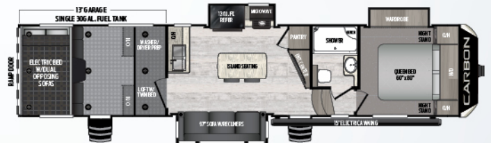
348 | 13' garage, island w/seating, tandem axle Weight: 12535 lbs | Length: 38' 11"
