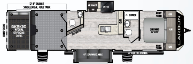
36 | L-shaped kitchen, 12' garage, angled entertainment Weight: 9990 lbs | Length: 38'
