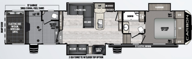
403 | L-shaped sofa, 1 1/2 bath, triple axle, 13' garage Weight: 14270 lbs | Length: 43' 6"
