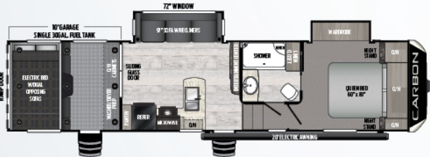
337 | Tandem axle, two slides, 10' garage Weight: 11760 lbs | Length: 35' 11"
