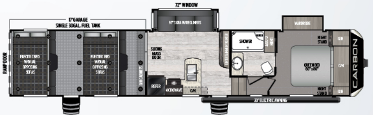
387 | Triple axle, two slides, 17' garage Weight: 13380 lbs | Length: 42' 8"
