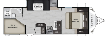
KODIAK ULTRA-LITE 248BHSL Length: 28' 11" Weight: 5,298lbs Sleeps: 6-8 Hitch: 584 lbs. Height: 10'7"
