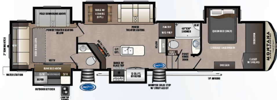
362RD | REAR DEN OR REAR BUNKHOUSE | Weight: 13097 LBS. | Length: 40' 1" RV REFRIGERATOR
