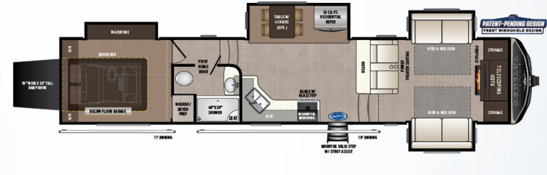
380/381TH | FRONT LIVING ROOM W/ REAR GARAGE AND RAMP DOOR | WEIGHT: 13546 LBS. | LENGTH: 41' 6" RV REFRIGERATOR | RES. REFRIGERATOR
