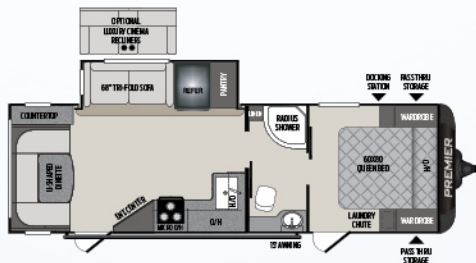
26UDPR | Rear dinette, dual entry Weight: 5519 | Length: 30' 11"
