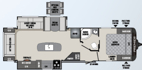
30RIPR | Rear living, island kitchen, outside entertainment Weight: 6871 LBS. | Length: 35' 11"
