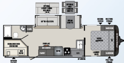
29BHPR | Bunkhouse, outside kitchen Weight: 6000 LBS. | Length: 33' 4"
