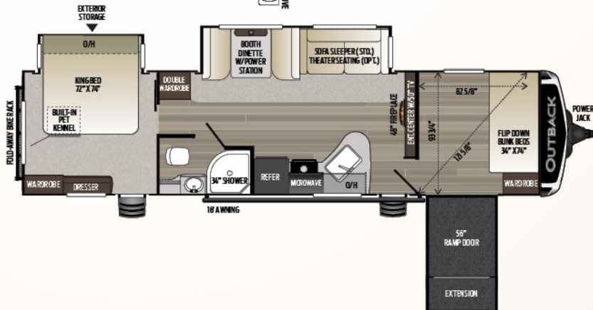
Cargo garage, two slides Weight: 8006 LBS. | Length: 37'4"
