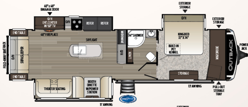
Rear living, three slides-inc. bedroom Weight: 8718 LBS. | Length: 37'10"
