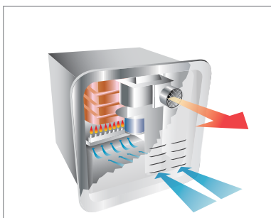
OPTIONAL GIRARD 3RD-GENERATION TANKLESS WATER HEATER WITH DIGITAL THERMOSTAT
