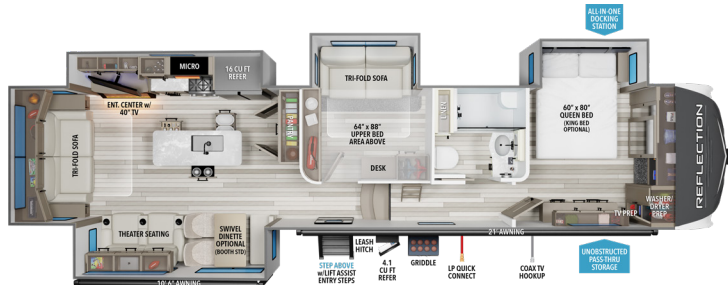
UVW 1 HITCH 1 LENGTH 2 HEIGHT 3 CAPACITY 367BHS 12,900 2,550 41' 1" 12' 8" 74 78 39
