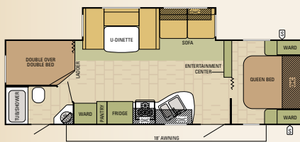
25BHS | AR-ONE MAXX
