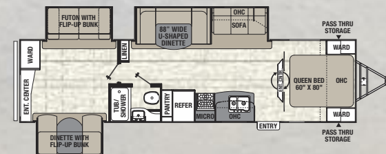
312 BHDS ♦ Exterior Length 36' 9"
