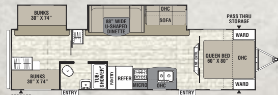
31 SE ♦ Exterior Length 35' 7"
