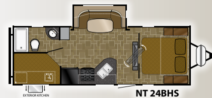
Length: 27' 11" Dry: 5,585 NT 24BHS Height: 11' 2" Hitch: 550 GVWR: 6,900
