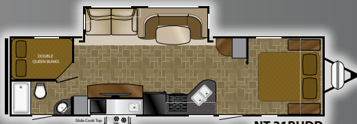
Length: 35' 11" Dry: 6,399 NT 31BHDD Height: 11' 4" Hitch: 652 GVWR: 8,600
