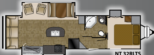
Length: 36' 8" Dry: 6,950 NT 32RLTS Height: 11' 4" Hitch: 780 GVWR: 8,600
