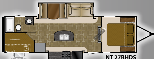
Length: 32' 8" Dry: 6,674 NT 27BHDS Height: 11' 4" Hitch: 780 GVWR: 8,600
