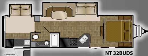
Length: 35' 10" Dry: 6,795 NT 32BUDS Height: 11' 4" Hitch: 655 GVWR: 8,600
