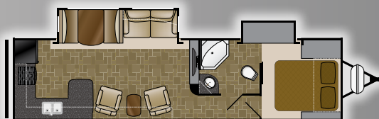
Length: 36' 9" Dry: 6,795 NT 30RKDD Height: 11' 4" Hitch: 788 GVWR: 8,600
