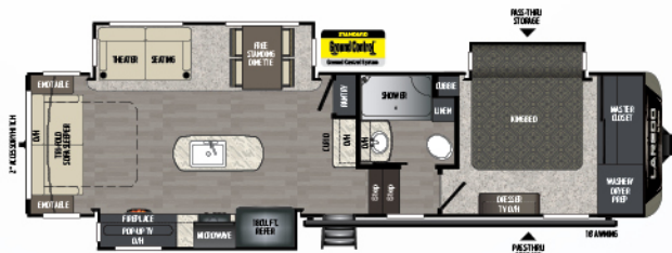
310RS | Rear living room, triple slide, king bed Weight: 10479 lbs | Length: 35' 1"
