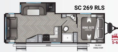
Length 30' 11" Dry 5,832 lbs. Hitch 820 lbs. Height 10' 11"
