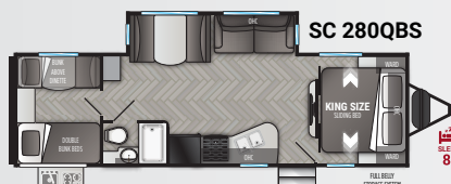
Length 31' 11" Dry 6,288 lbs. Hitch 816 lbs. Height 10' 11"
