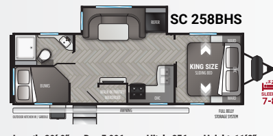
Length 29' 9" Dry 5,996 lbs. Hitch 856 lbs. Height 11' 2"
