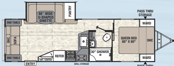
279 RLSLE / Exterior Length 31' 11"
