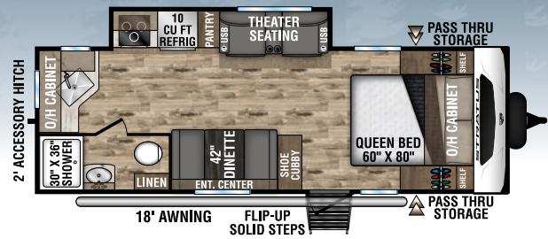
SR241VRK | TBD UVW | 26' 10" LENGTH | SLEEPS 4
